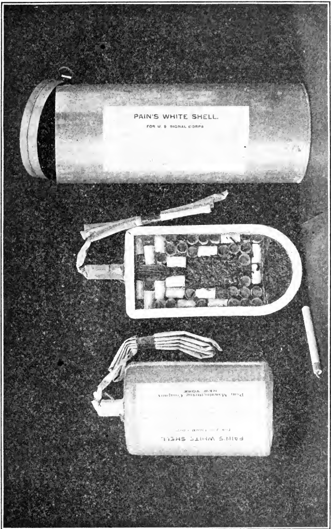
FIG. 12.—Signaling shells.
